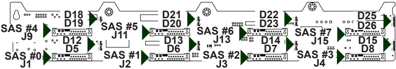
Figure 2-5: Rear Connectors and LEDs
