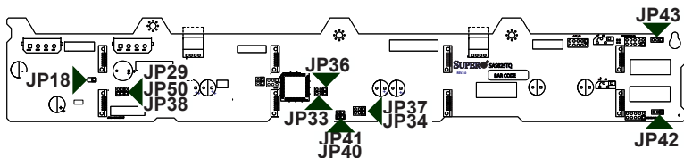
Figure 2-3: Front Jumpers
