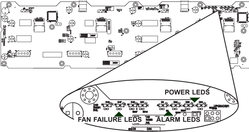
Figure 2-3: Front LEDs
