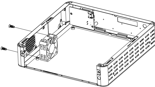
Figure 4-5. System Fan
