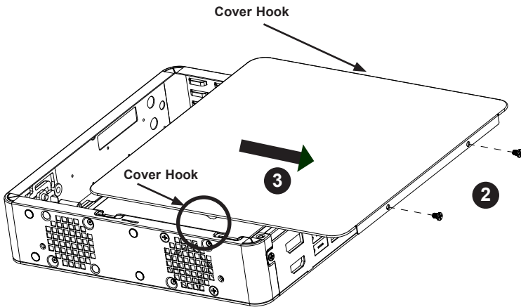
Figure 4-1. Removing the Chassis Cover
