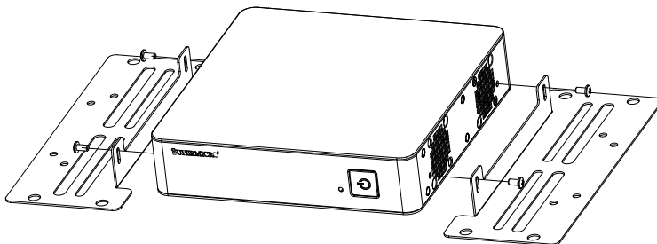
Figure 4-3. Installing Mounting Brackets (Configuration B Shown)
