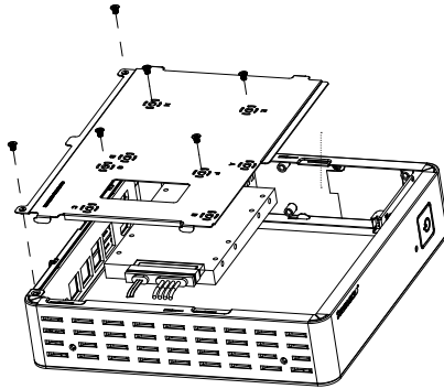
Figure 4-4. Installing the Hard Drive
