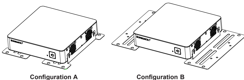
Figure 4-2. Mounting Bracket Configuration Options
