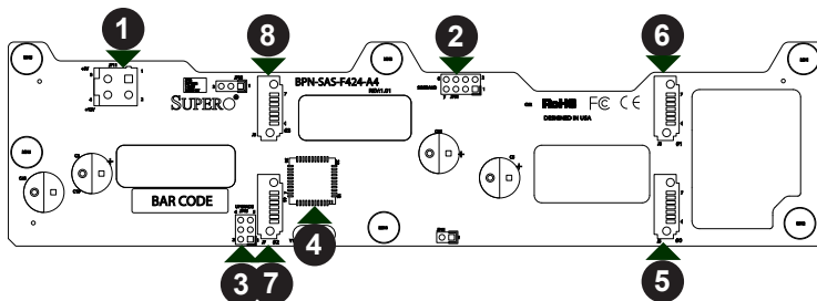
Figure 2-1: Front Connectors
